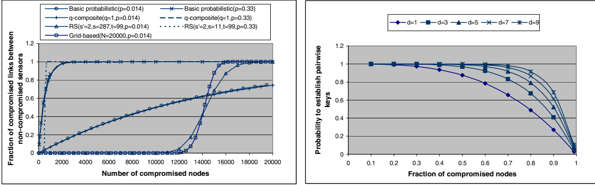
(a) Fraction of compromised links between non-compromised sensors v.s. number of compromised sensor nodes. Assume each sensor has available storage equivalent to 200 keys.
